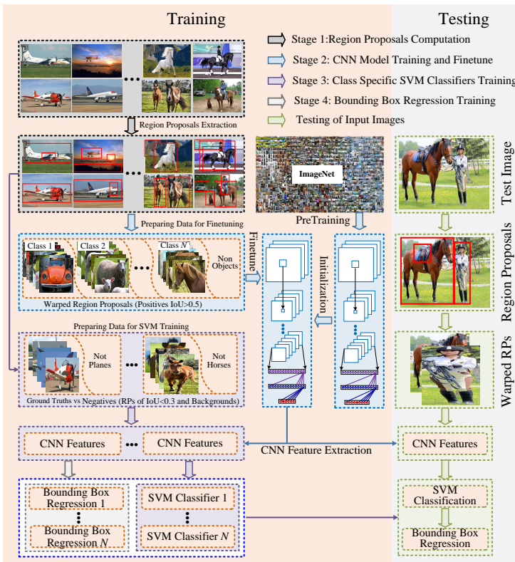
Fig. 7 Illustration of the milestone detecting framework RCNN [65, 67] in great detail.
