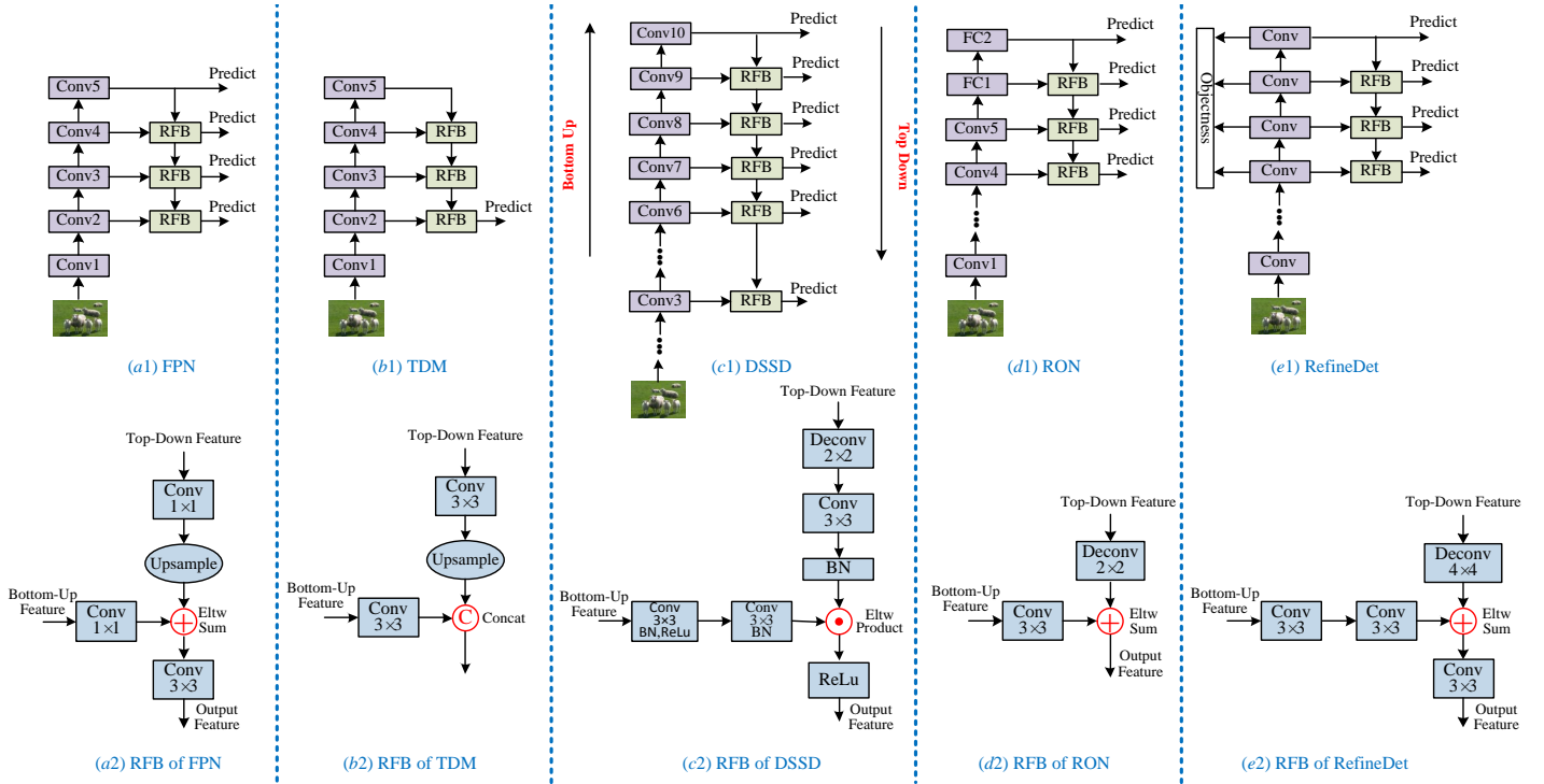
Fig. 11 Hourglass architectures: Conv1 to Conv5 are the main Conv blocks in backbone networks such as VGG or ResNet. Comparison of a number of Reverse Fusion Block (RFB) commonly used in recent approaches.
