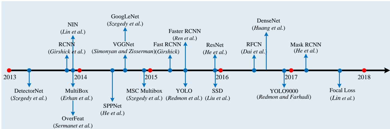
Fig. 6 Milestones in generic object detection based on the point in time of the first arXiv version.
