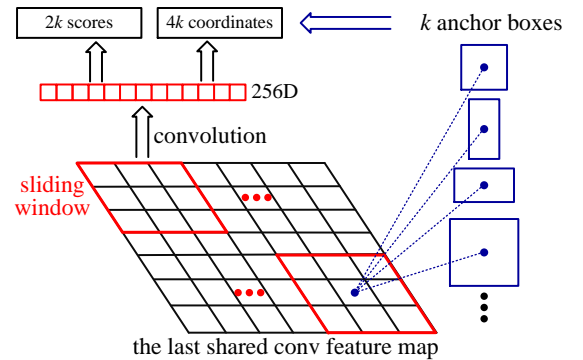
Fig. 14 Illustration of the Region Proposal Network (RPN) proposed in [175].
