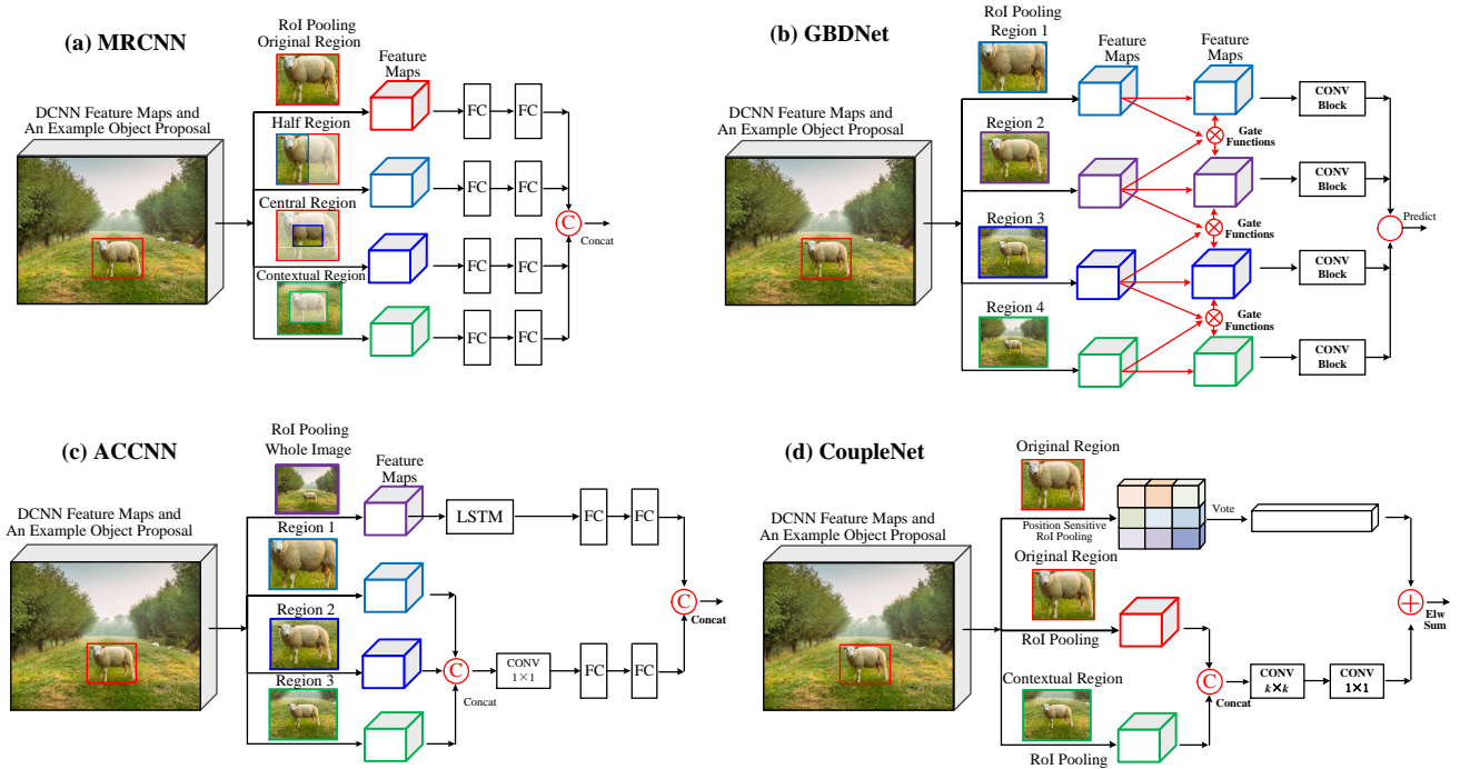
Fig. 13 Representative approaches that explore local surrounding contextual features: MRCNN [62], GBDNet [235, 236], ACCNN [123] and CoupleNet [251], see also Table 4.
