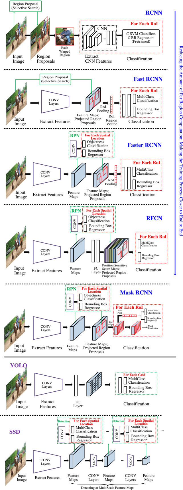
Fig. 8 High level diagrams of the leading frameworks for generic object detection. The properties of these methods are summarized in Table 10.
