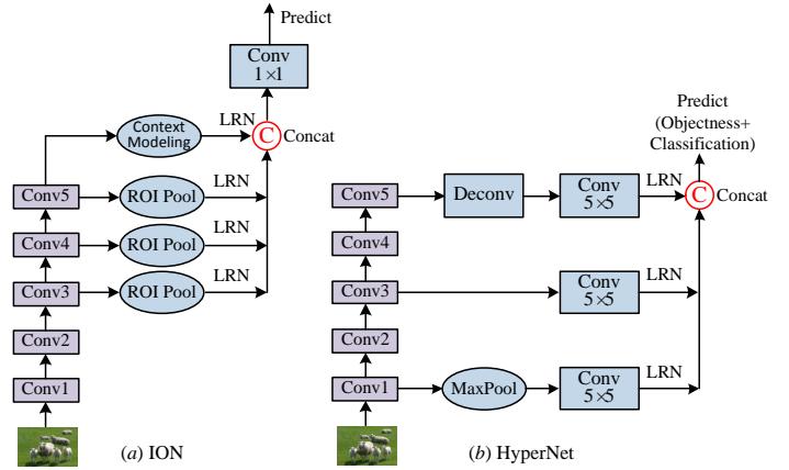
Fig. 10 Comparison of HyperNet and ION. LRN: Local Response Normalization
