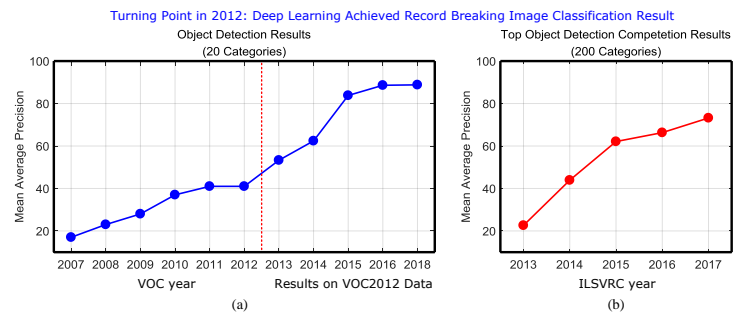
Fig. 1 Recent evolution of object detection performance. We can observe significant performance (mean average precision) improvement since deep learning entered the scene in 2012. The performance of the best detector has been steadily increasing by a significant amount on a yearly basis. (a) Results on the PASCAL VOC datasets: Detection results of winning entries in the VOC2007-2012 competitions (using only provided training data). (b) Top object detection competition results in ILSVRC2013-2017 (using only provided training data).
