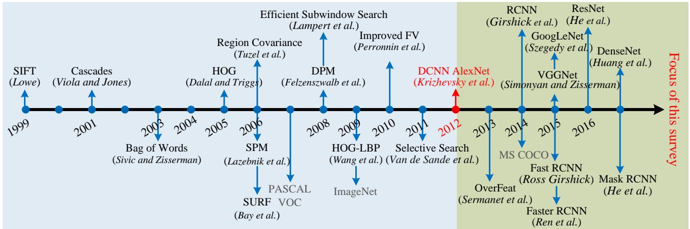
Fig. 2 Milestones of object detection and recognition, including feature representations [37, 42, 79, 109, 114, 139, 140, 166, 191, 194, 200, 213, 215], detection frameworks [56, 65, 183, 209, 213], and datasets [53, 129, 179]. The time period up to 2012 is dominated by handcrafted features. We see a turning point in 2012 with the development of DCNNs for image classification by Krizhevsky et al. [109]. Most listed methods are highly cited and won one of the major ICCV or CVPR prizes. See Section 2.3 for details.
