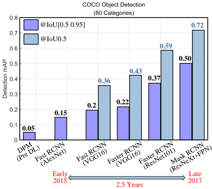
Fig. 17 Evolution of object detection performance on COCO (Test-Dev results). Results are quoted from [64, 80, 176] accordingly. The backbone network, the design of detection framework and the availability of good and large scale datasets are the three most important factors in detection.
